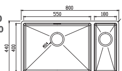
Jazz 1.5 bowl Ref. JA022LH LH Main Bowl £500 Ref. JA022RH RH Main Bowl £500 Overall size: 800/440 mm Bowl size: 550/400/190 mm Half bowl: 180/400/125 mm Minimum cabinet size: 800 mm
