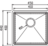
Jazz Single bowl Ref. JA012 £274 Overall size: 450/440 mm Bowl size: 410/400/190 mm Min cabinet size: 450 mm
