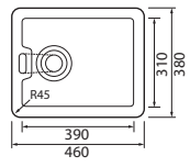
Belfast Mini Single bowl Ref. TBE460 White £458 Installation: Apron Front Overall size: 460/380/205 mm Bowl size: 390/310/180 mm Overflow: Yes Tap-holes: No
