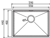
Jazz Single bowl Ref. JA013 £314 Overall size: 590/440 mm Bowl size: 550/400/190 mm Min cabinet size: 600 mm
