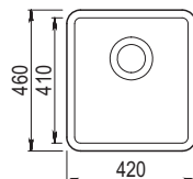
Nova Single bowl Ref. NOV N370 £299 Overall size: 420/460 mm Bowl size: 370/410/200 mm Cutout size: Template Available Minimum cabinet size: 450 mm Standard waste kit included
