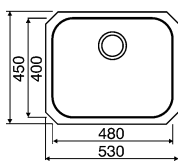
Tango Single bowl Ref. SP480 £240 Overall size: 530/450 mm Bowl size: 480/400/195 mm Minimum cabinet size: 600 mm
