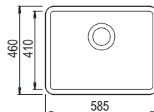
Nova Single bowl Ref. NOV N535 £339 Overall size: 585/460 mm Bowl size: 535/410/210 mm Cutout size: Template Available Minimum cabinet size: 800 mm Standard waste kit included
