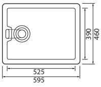
Belfast Single bowl Ref. TBE600 White £483 Installation: Apron Front Overall size: 595/460/255 mm Bowl size: 525/390/217 mm Overflow: Yes Tap-holes: No
