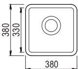
Nova Single bowl Ref. NOV N330 £279 Overall size: 380/380 mm Bowl size: 330/330/190 mm Cutout size: Template Available Minimum cabinet size: 450 mm Standard waste kit included
