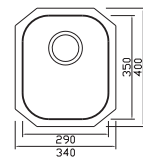
Tango Single bowl Ref. SP350 £140 Overall size: 340/400 mm Bowl size: 290/350/165 mm Minimum cabinet size: 400 mm
