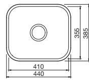
Tango Single bowl Ref. SP410 £190 Overall size: 440/385 mm Bowl size: 410/355/180 mm Minimum cabinet size: 450 mm
