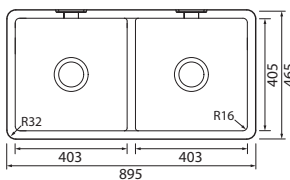
Wessex Double bowl Ref. TWE900 White £918 Installation: Apron Front Overall size: 895/465/229 mm Bowl sizes: 403/405/199 mm Overflow: Yes Tap-holes: No
