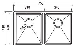
Jazz Double bowl Ref. JA024 £500 Overall size: 750/440 mm Bowl sizes: 340/400/190 mm Minimum cabinet size: 800 mm
