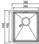
Jazz Single bowl Ref. JA014 £248 Overall size: 380/440 mm Bowl size: 340/400/190 mm Min cabinet size: 400 mm
