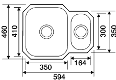
Tango 1.5 bowl (Reversible) Ref. SP20 £260 Overall size: 594/460 mm Bowl size: 350/410/185 mm Half bowl: 164/300 mm Minimum cabinet size: 600 mm
