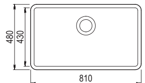
Nova Single bowl Ref. NOV N780 £439 Overall size: 810/480 mm Bowl size: 760/430/230 mm Cutout size: Template Available Minimum cabinet size: 1000 mm Standard waste kit included
