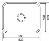
Tango Single bowl Ref. SP500 £260 Overall size: 533/433 mm Bowl size: 500/400/200 mm Minimum cabinet size: 600 mm
